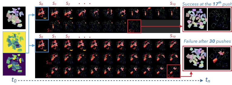
Fig. 4: A qualitative example of mask prediction during two testing episodes in Task no 1 in Condition 2 (Push-To-See M2 in upper panel, Heuristic baseline in lower panel). The figure shows how the consecutive pushes decreases the segmentation error of the scene after each interaction. At the initial state s_0 , both Mask-RG models receive the same depth and GT images. Red coloured objects are the false negatives (FN). Whilst Push-To-See successfully completes the episode by detecting all of the initial 15 FNs at s_0 after 17 conducting pushes, the heuristic baseline fails to succeed in this episode. After 30 pushing trials, the baseline decreases the number of FNs from 15 to 5 at s_{30} .
