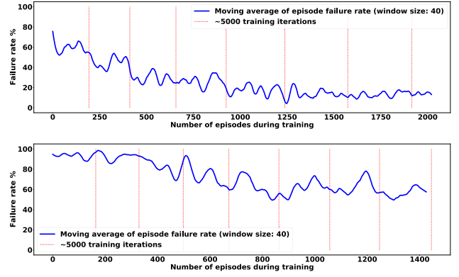
Fig. 3: Moving average of the episode failure rates during two model trainings (window size: 40). (The training curves have been smoothed out for printing by a Savitzky–Golay filter.). Upper panel shows the failure rate of Push-to-See (M1) during training in Condition 1, whilst lower panel is the training of Push-to-See (M2) in Condition 3. Red vertical lines indicate each 5000 \pm 30 training iterations. Since the episodes require more pushing actions at the beginning of the training, the distance between these lines are smaller.
