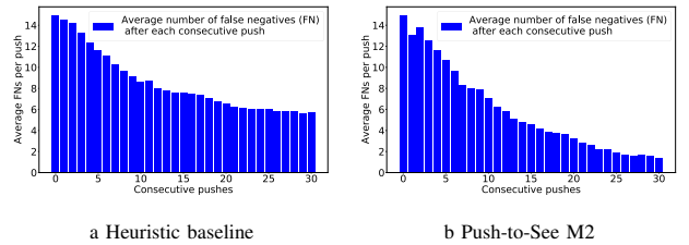
Fig. 6: Average number of false negatives (FN) per consecutive push in Task no.1 and Condition 2. When a task is solved after a push, the final FN score were carried for the remaining iterations in that episode for calculating the average.
