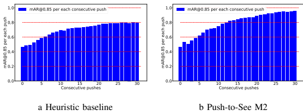
Fig. 5: Mean Average Recall @ 0.85 IoU in Task No 1 in Condition 2. Y axes indicate mAR@.85 scores for each particular push conducted one after another. When a task is solved after a push, the final mAR score were carried for the remaining iterations in that episode for calculating the average.
