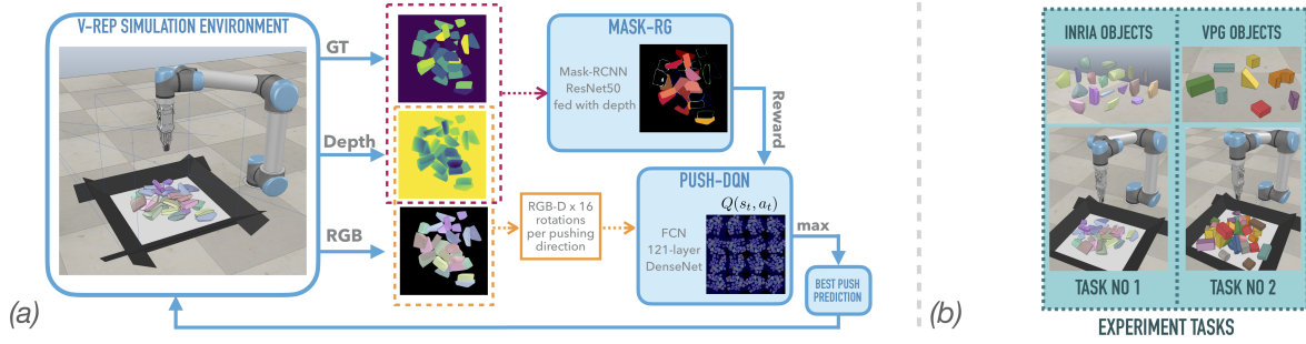
Fig. 2: (a) Overview of Push-to-See. Our model is two-fold: a Mask R-CNN based reward generator (Mask-RG) and a DQN based pushing predictor (Push-DQN). RGB, depth and ground truth (GT) segmentation masks are captured from the simulation environment. The depth and GT images are fed into Mask-RG in order to generate a segmentation score based on the difference in category-agnostic instance segmentation quality of the previous scene and the current scene. Meanwhile, 16 RGB-D heightmaps are generated from the depth and RGB to represent the current state-action value for 224 \times 224 \times 16 possible pushing actions similarly as in [1]. Push-DQN is then trained through trial and error by the reward signal to learn the best action-value pair (i.e. pushing action) which would enhance the instance segmentation of the consecutive scene. (b) Experimental setup consisting of 2 sets of objects from INRIA and VPG. Dense clutters include 28 objects in Task no 1 and 30 objects in Task no 2. Note the small depth variations in INRIA objects which makes their segmentation challenging. We employ only depth features for segmentation.
